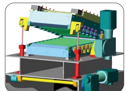
Digital servo-release
