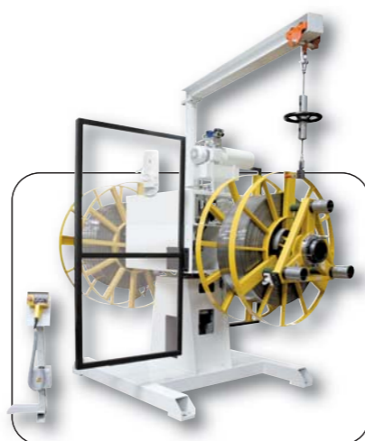
Double decoiler
