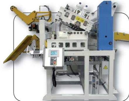
Cradle type straightener
