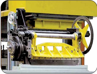
Mechanical guillotine shear
