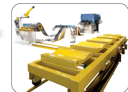
MULTICOIL
