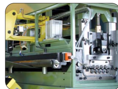
Straightener for thin strips
