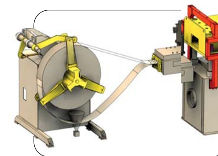
"3 in 1" line
