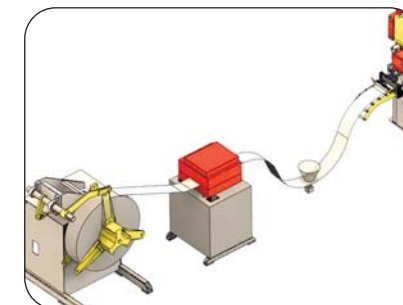
Long line
