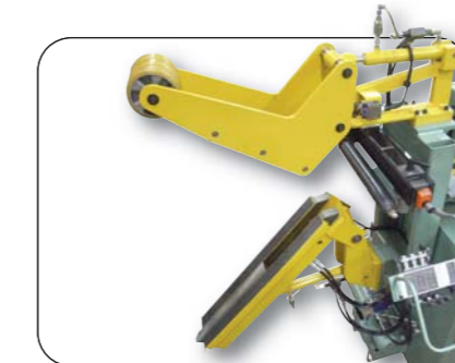
Threading peeler with 3 hydraulic movements
