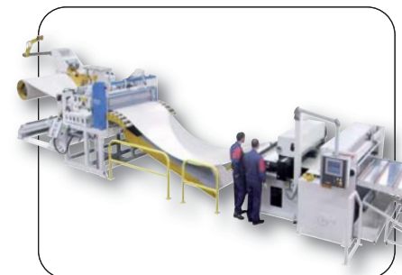
Cut-to-length line
