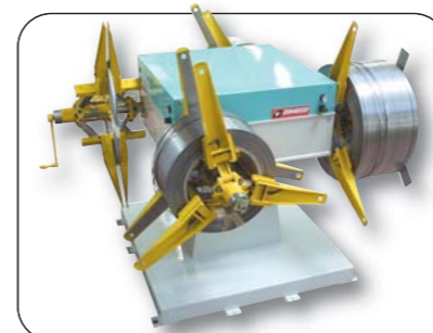
Quadruple decoiler for spool material
